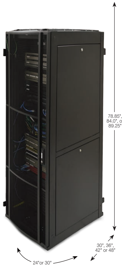
Part No. shown: XH7M451300000 (45RU x 30" W x 42" D)
